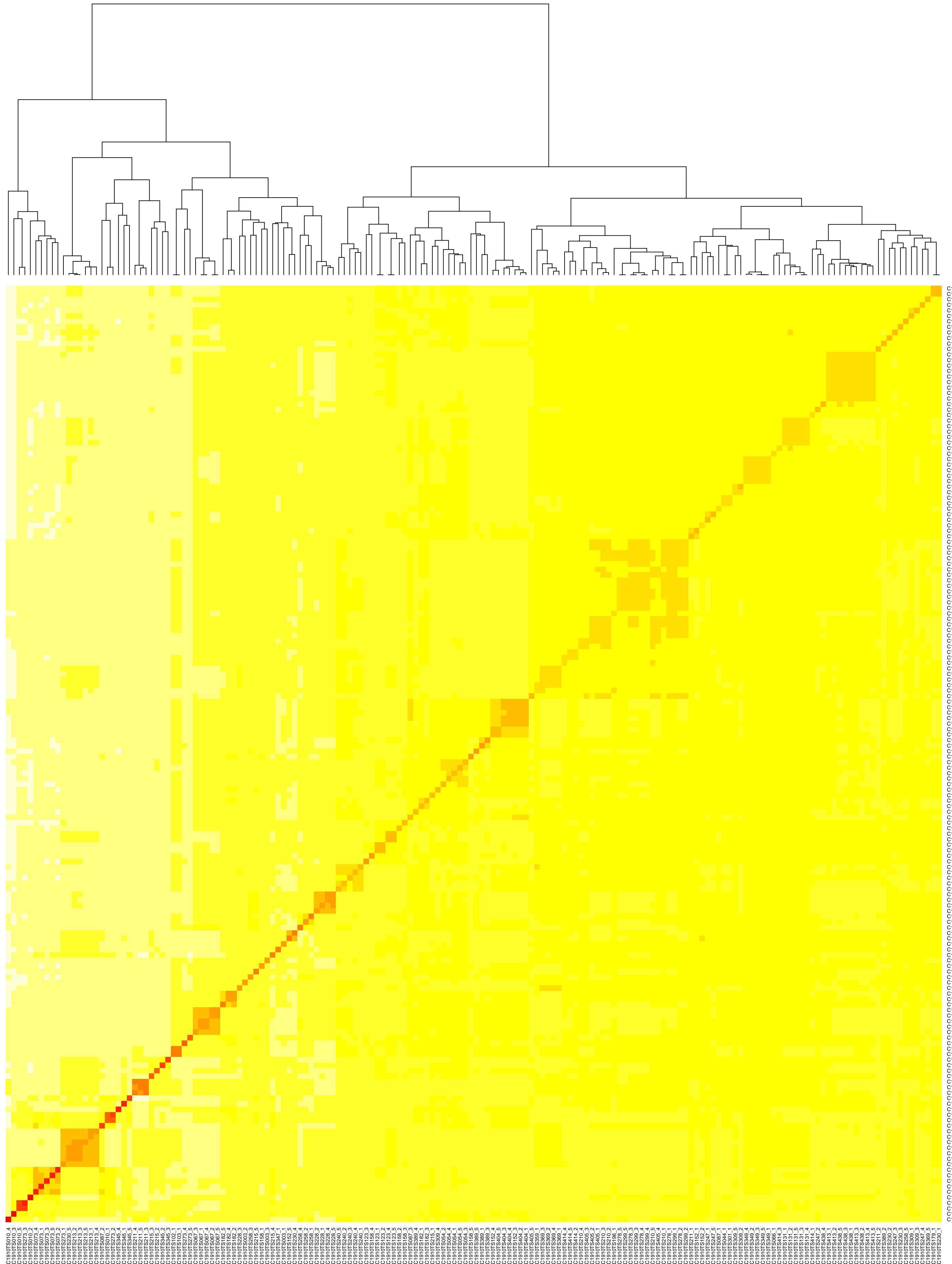
LDDT-based clustering heatmap for C1910
