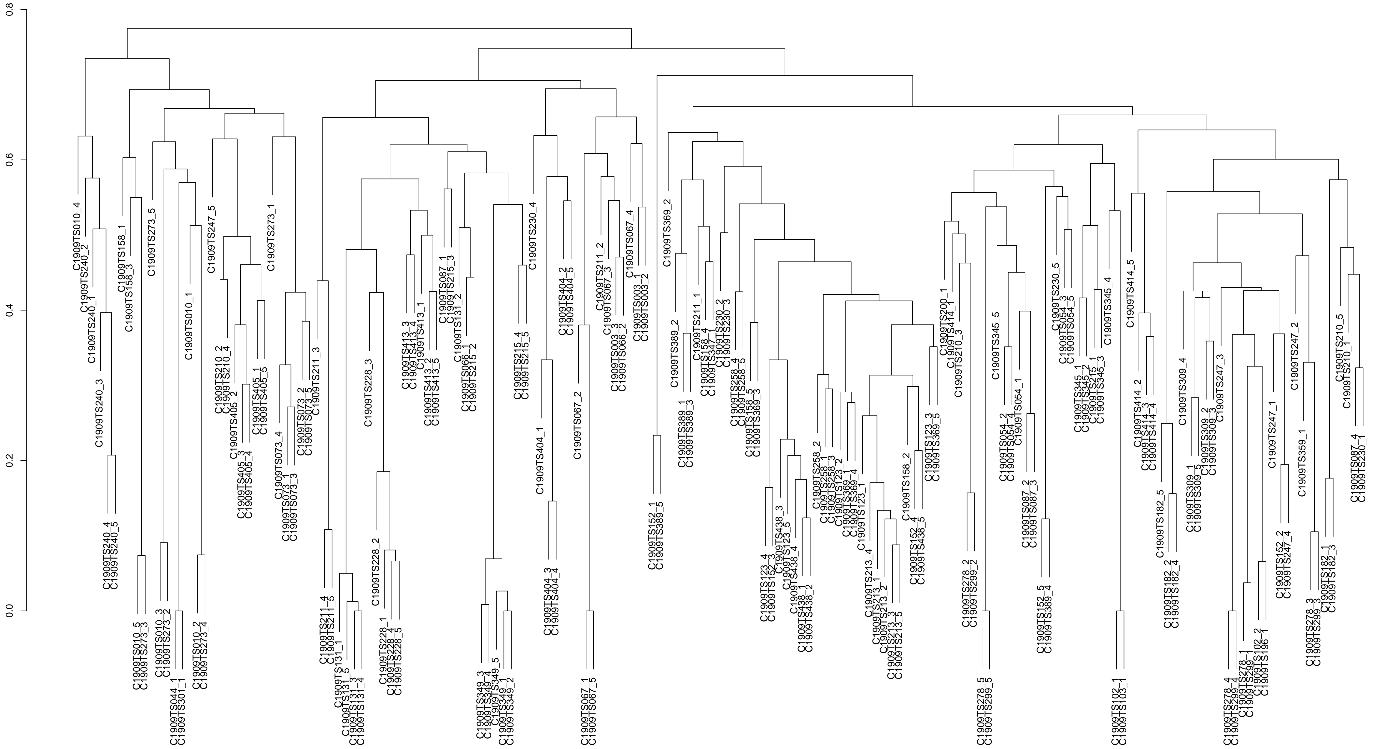
LDDT-based clustering dendrogram for C1909
