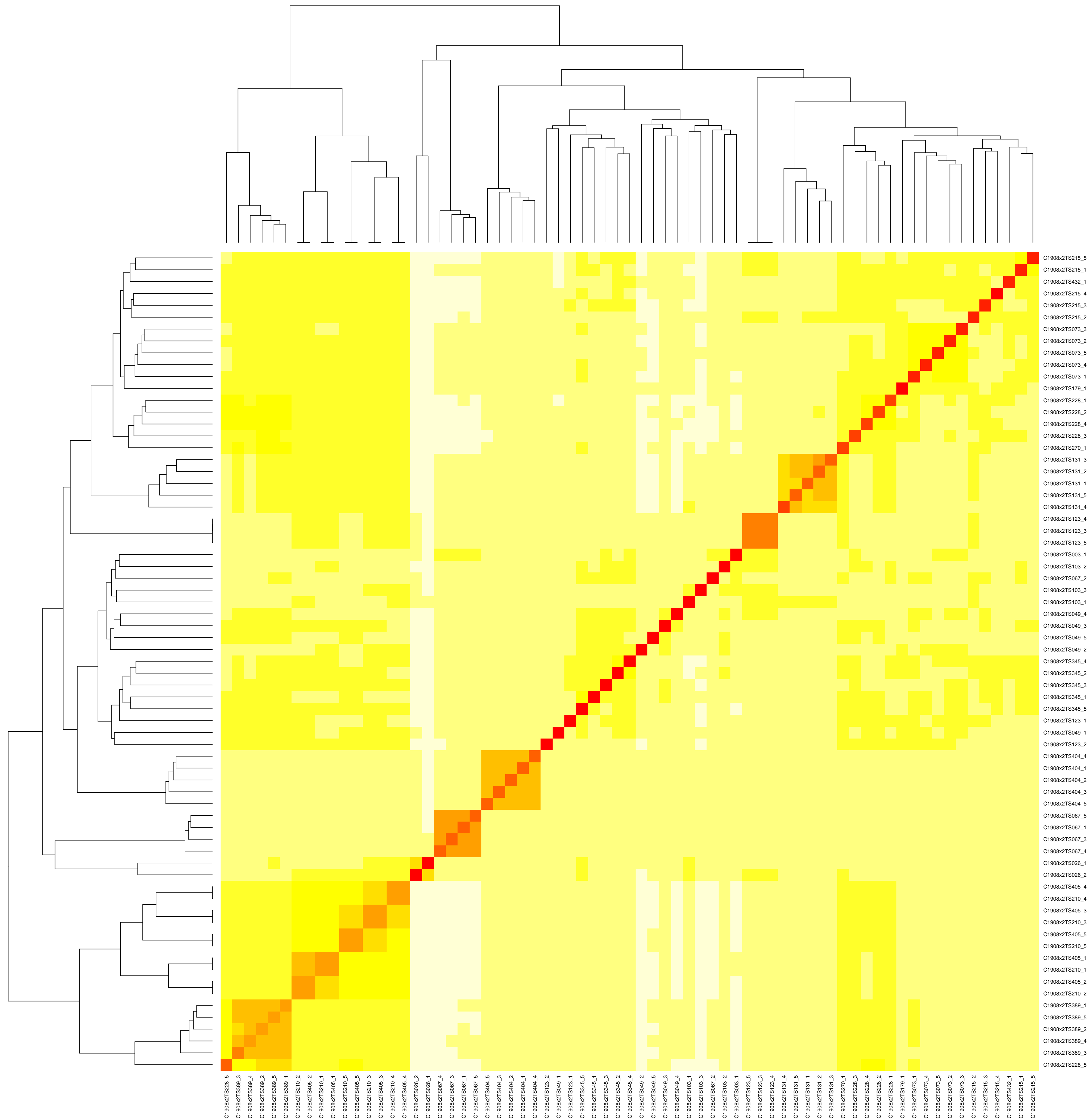
LDDT-based clustering heatmap for C1908x2
