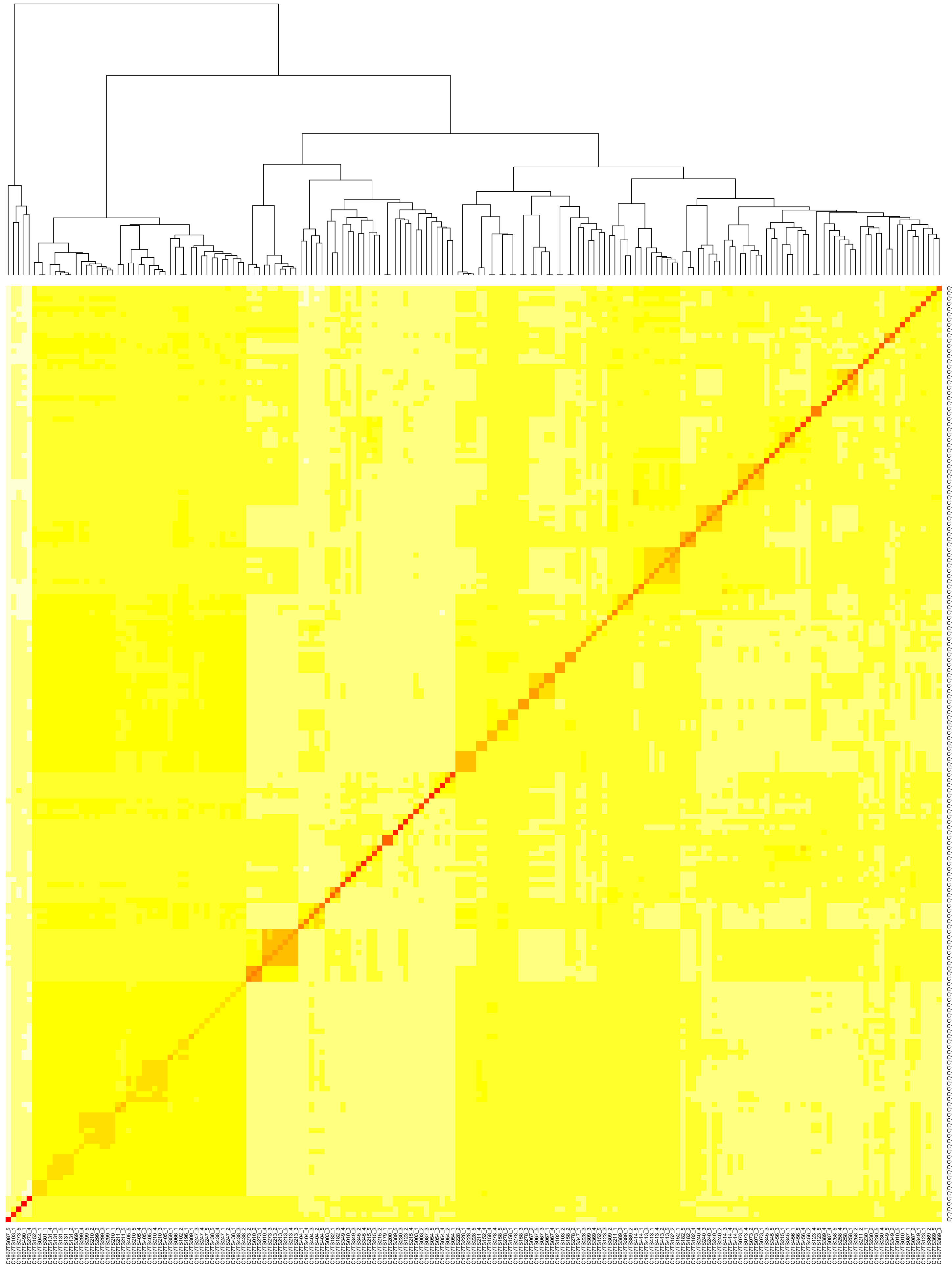
LDDT-based clustering heatmap for C1907
