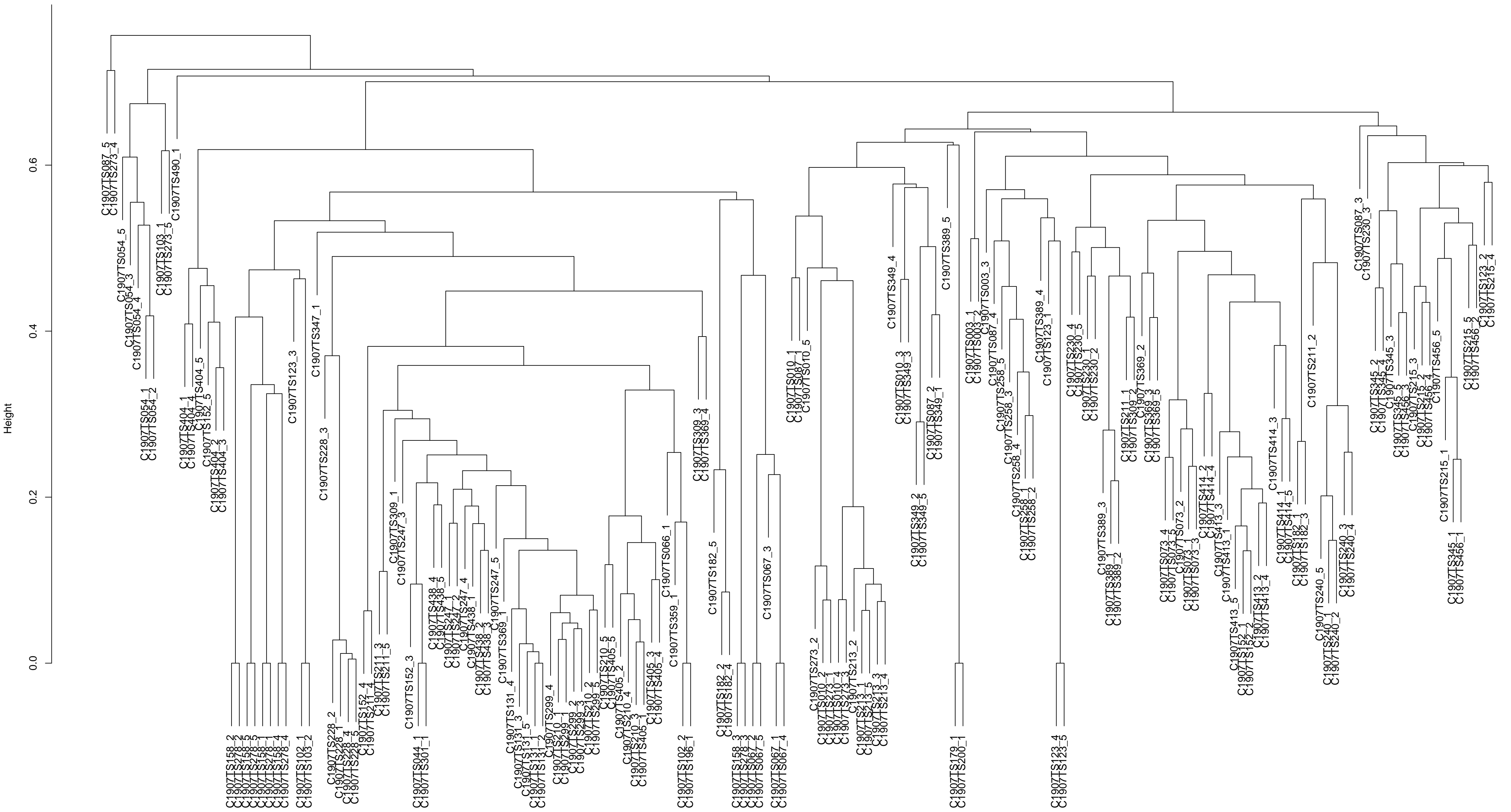
LDDT-based clustering dendrogram for C1907
