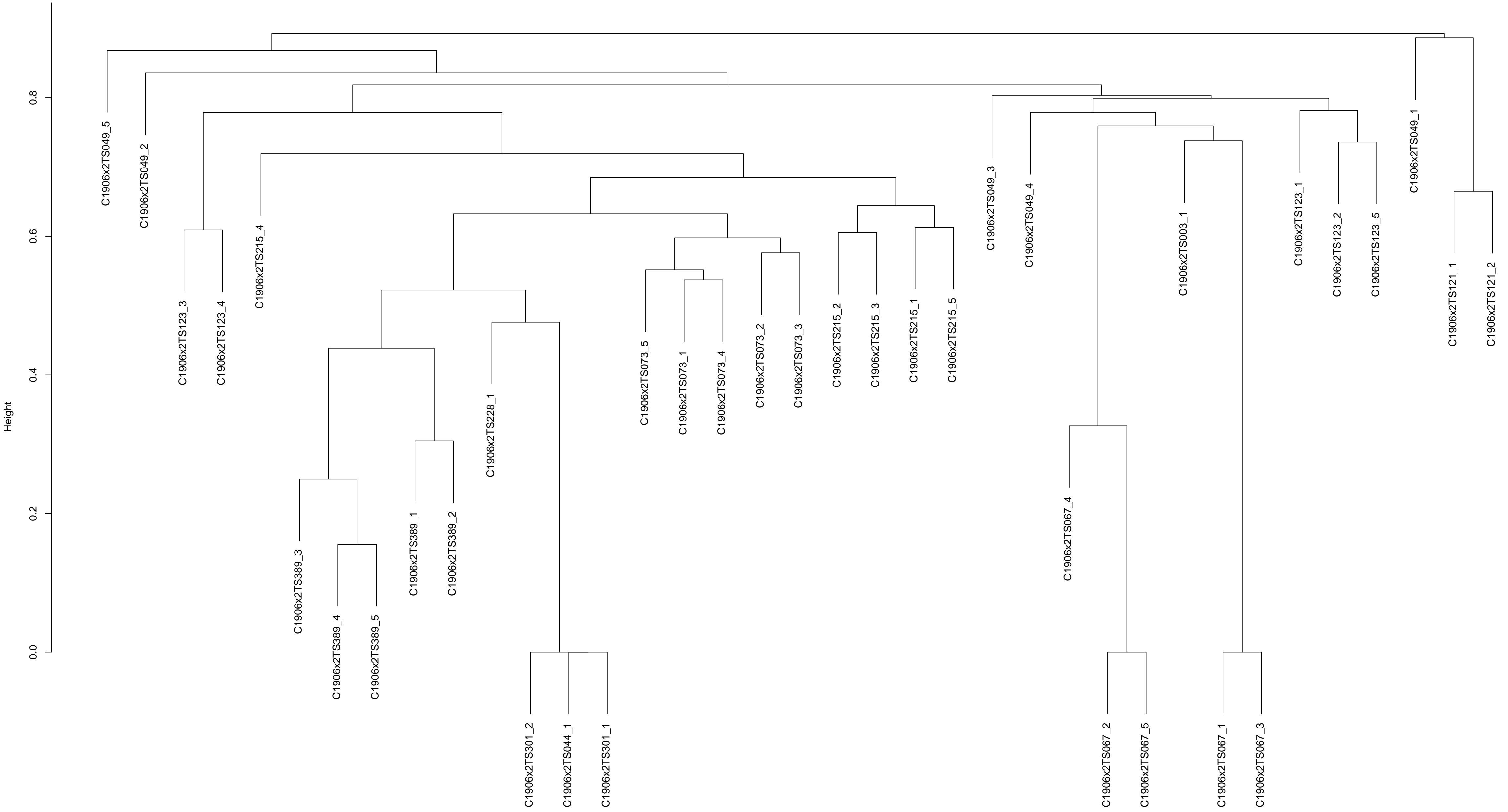
LDDT-based clustering dendrogram for C1906x2
