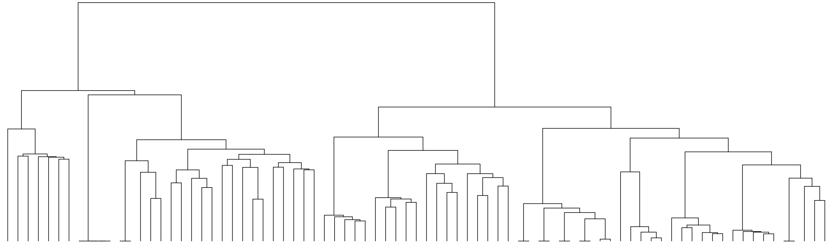
LDDT-based clustering heatmap for C1906d2
