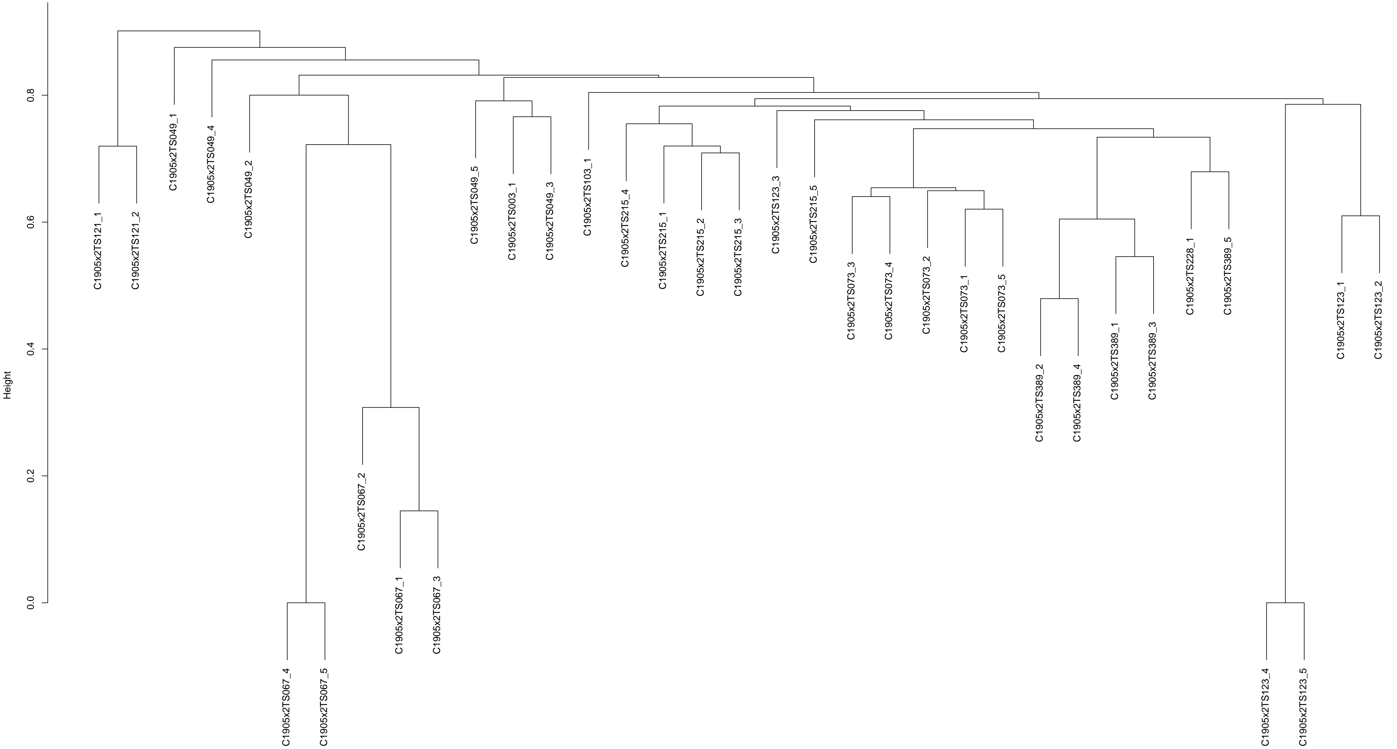
LDDT-based clustering dendrogram for C1905x2
