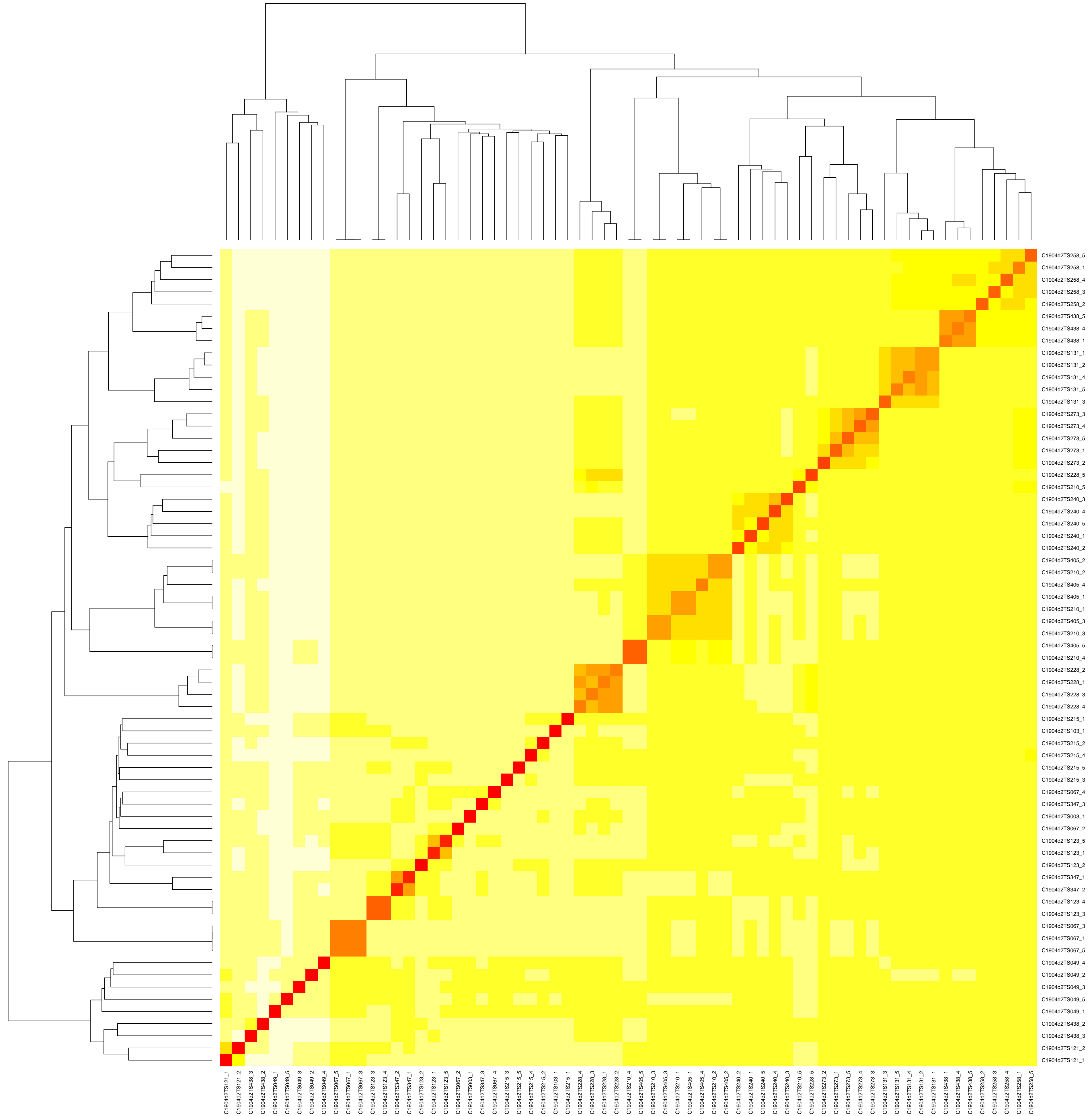
LDDT-based clustering heatmap for C1904d2
