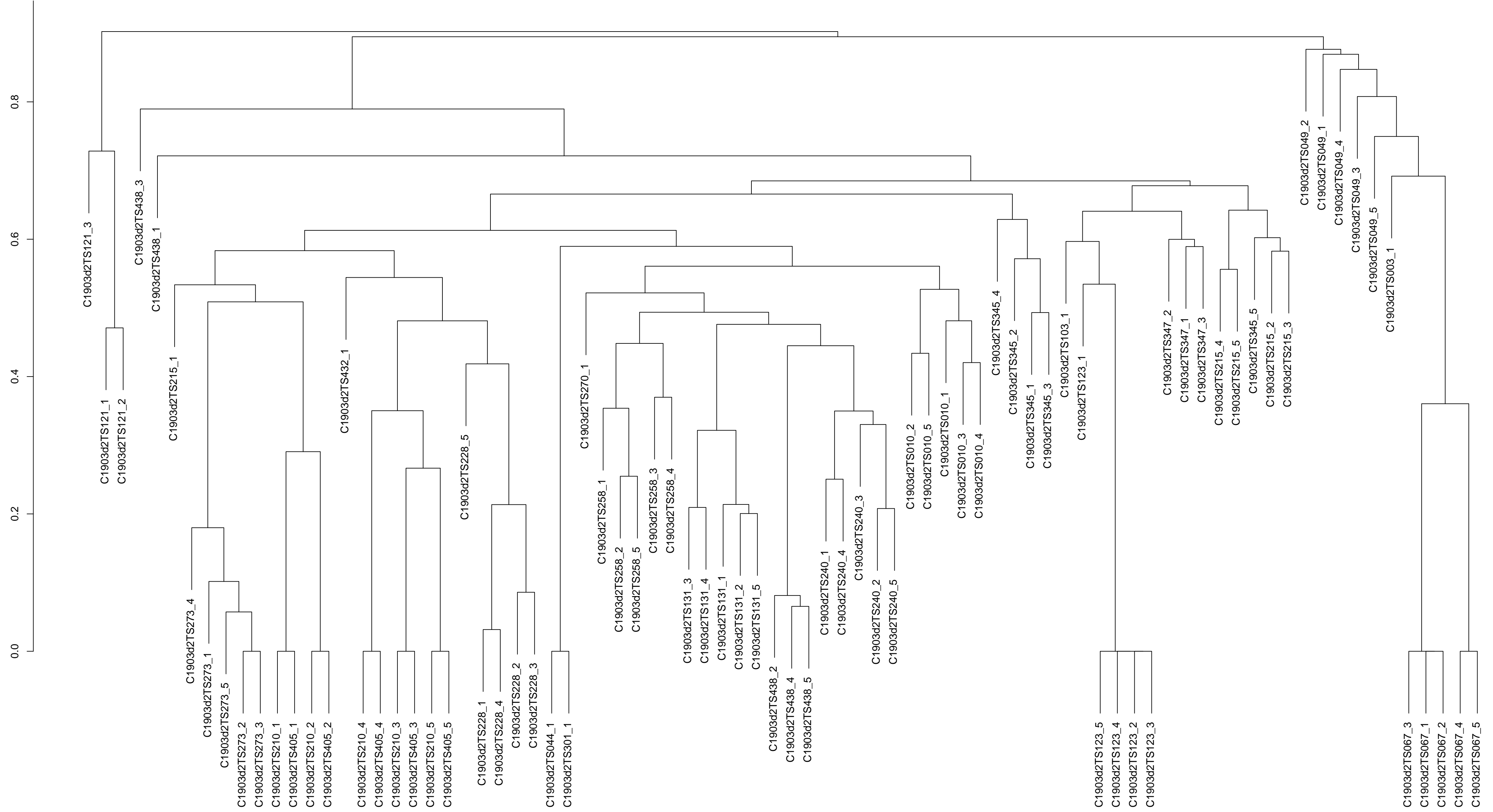
LDDT-based clustering dendrogram for C1903d2
