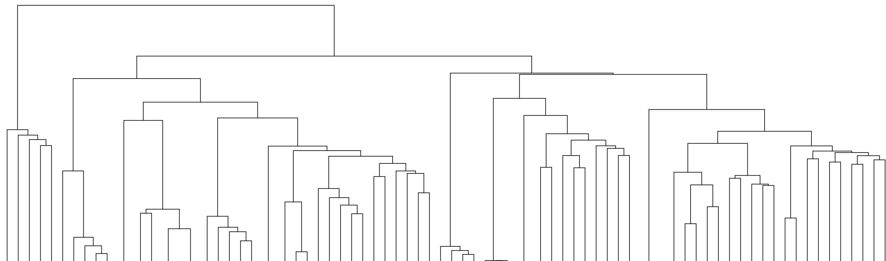
LDDT-based clustering heatmap for C1903d1
