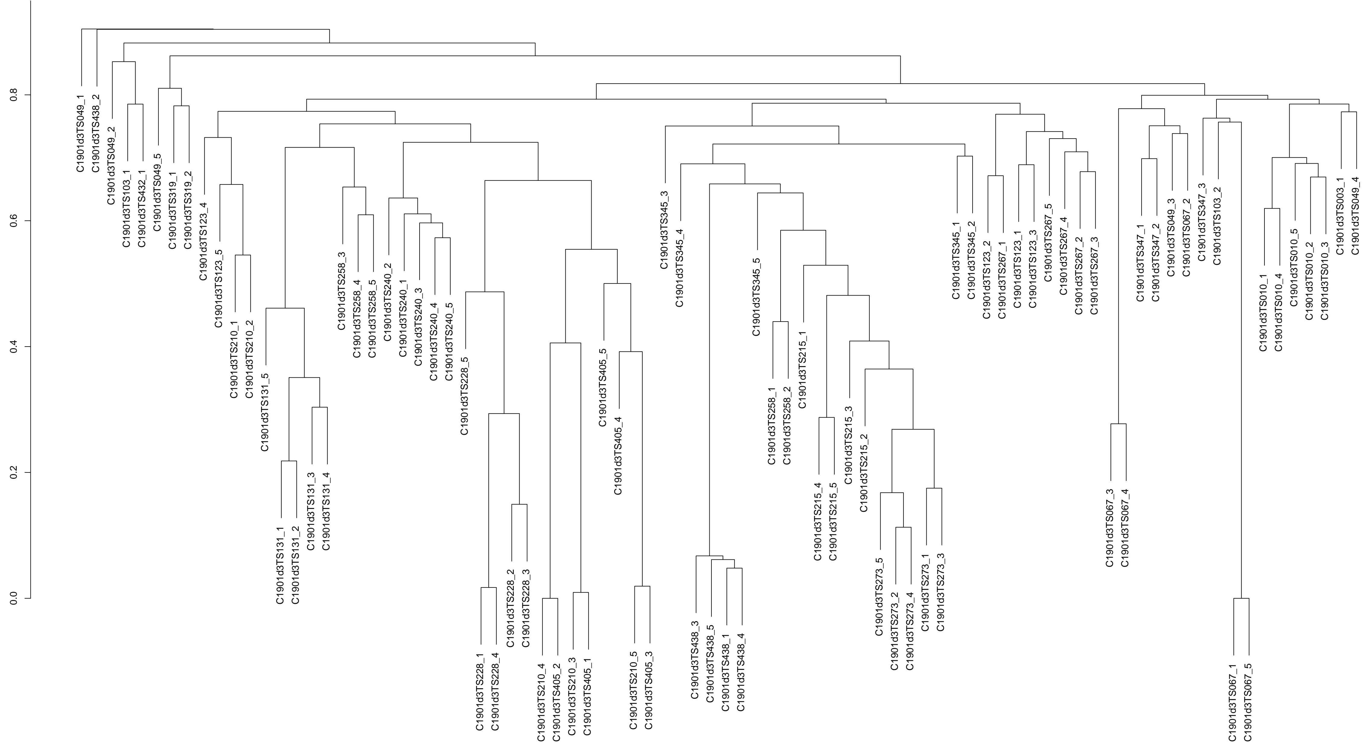
LDDT-based clustering dendrogram for C1901d3
