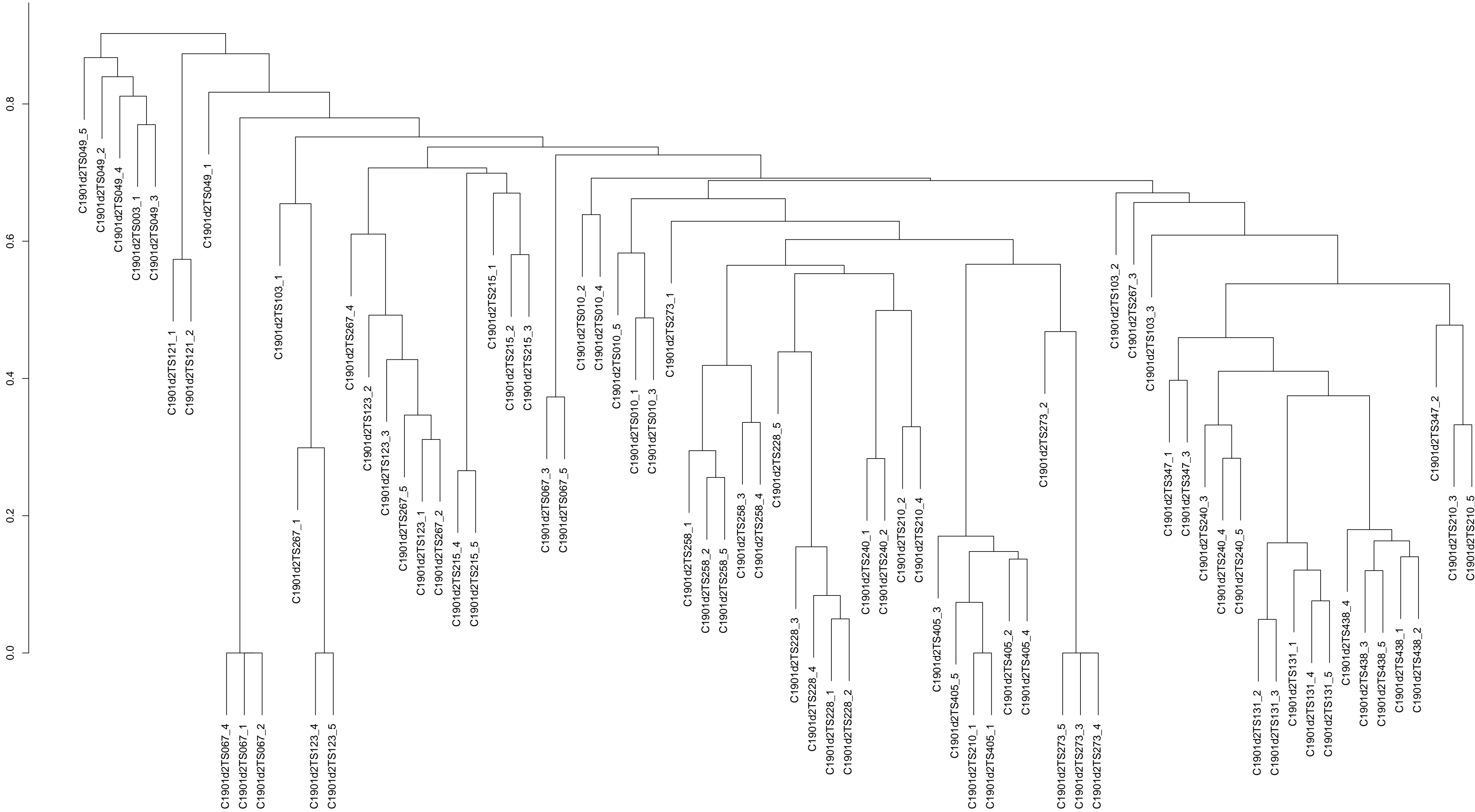
LDDT-based clustering dendrogram for C1901d2
