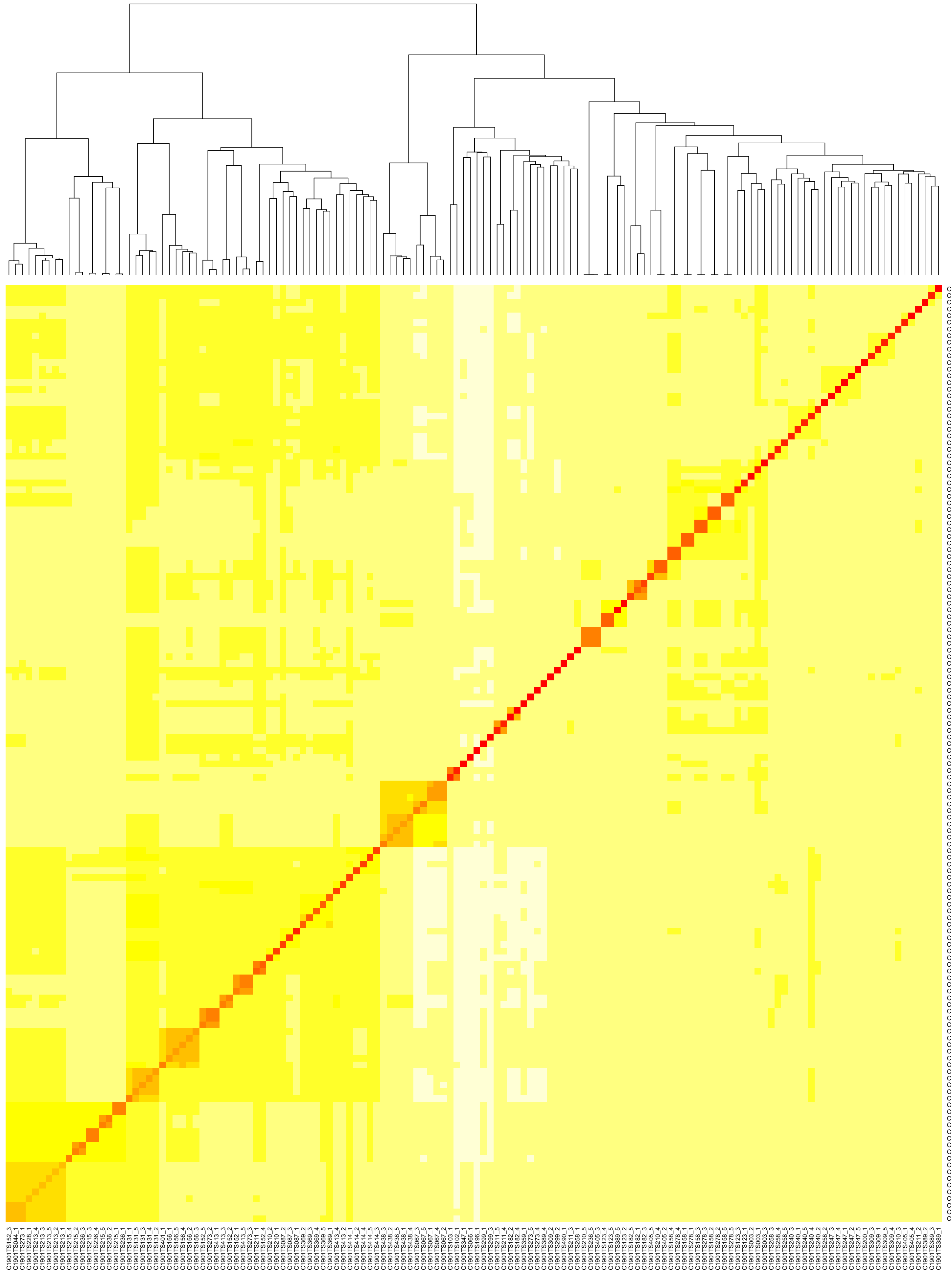
LDDT-based clustering heatmap for C1901
