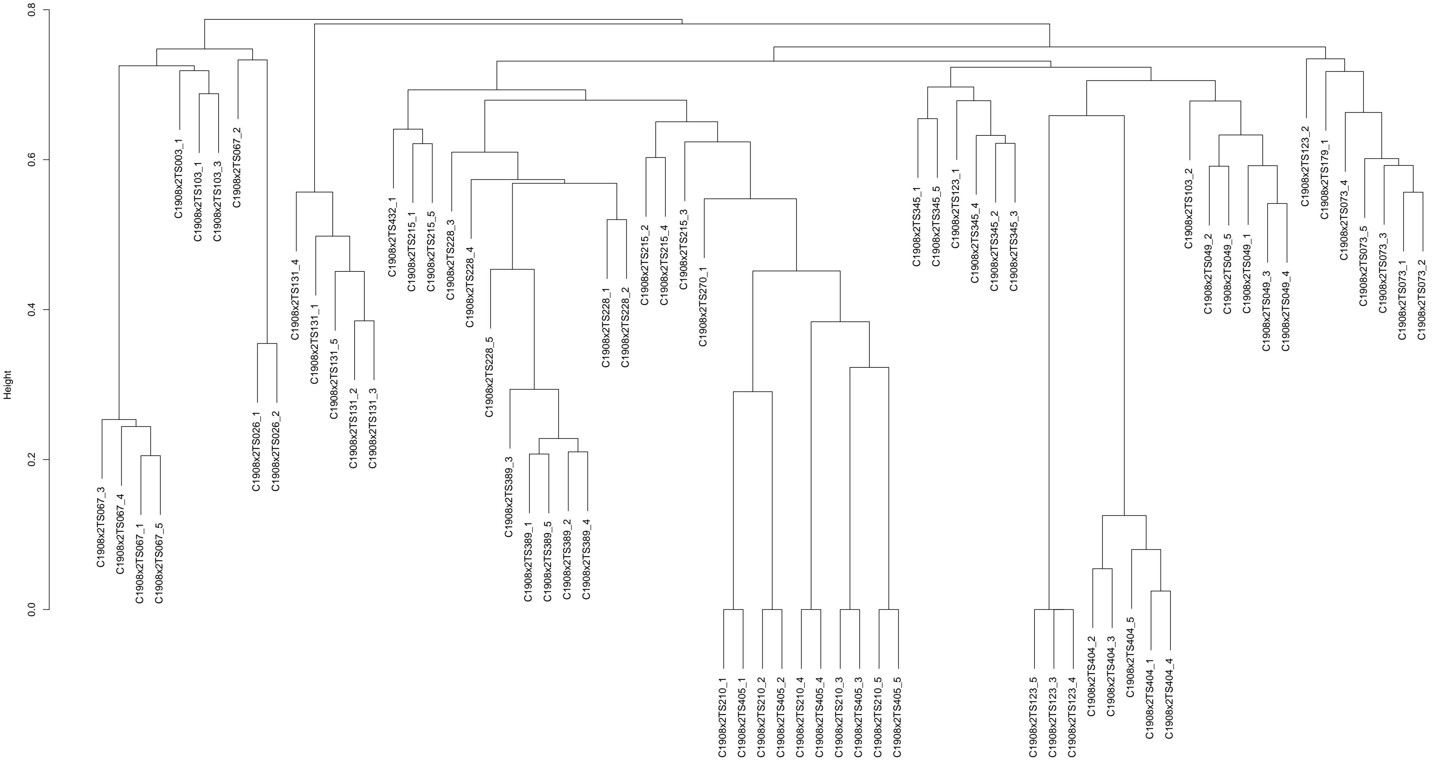
CAD-score-based clustering dendrogram for C1908x2
