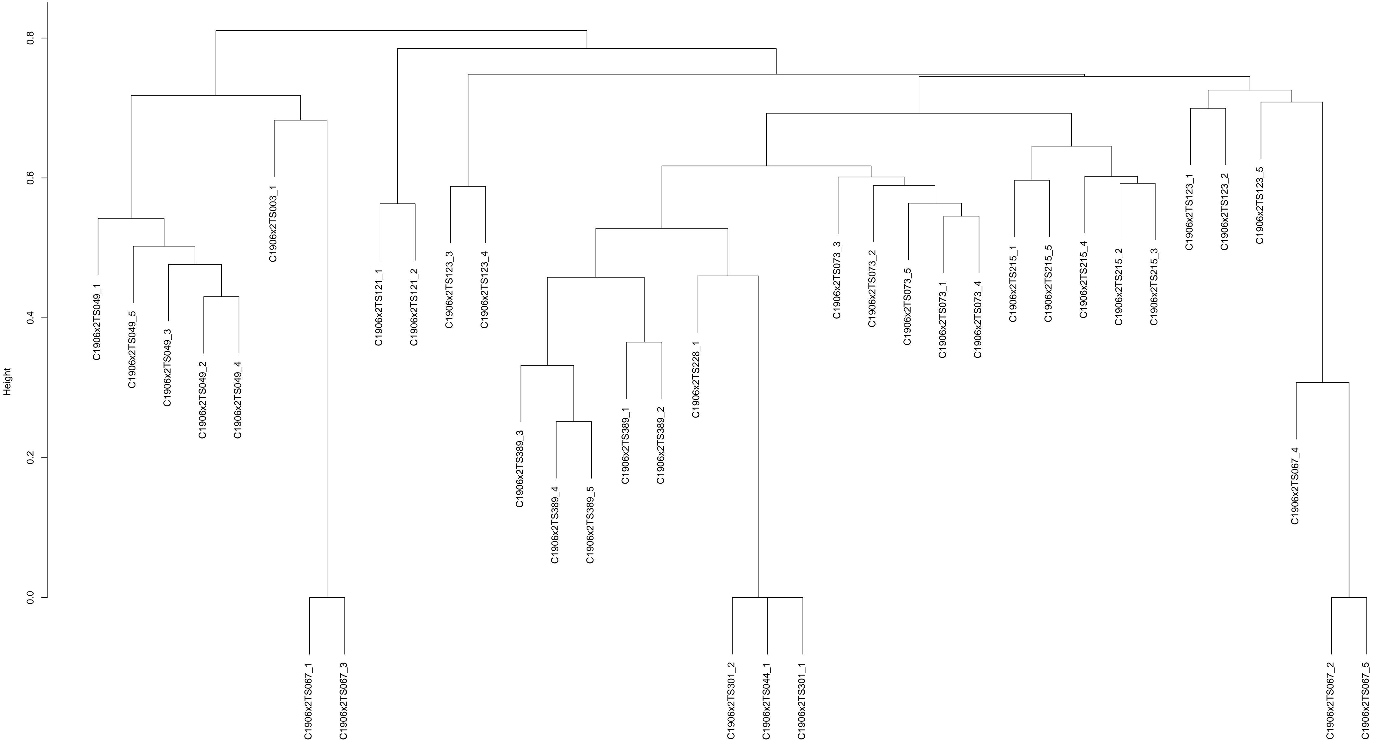
CAD-score-based clustering dendrogram for C1906x2
