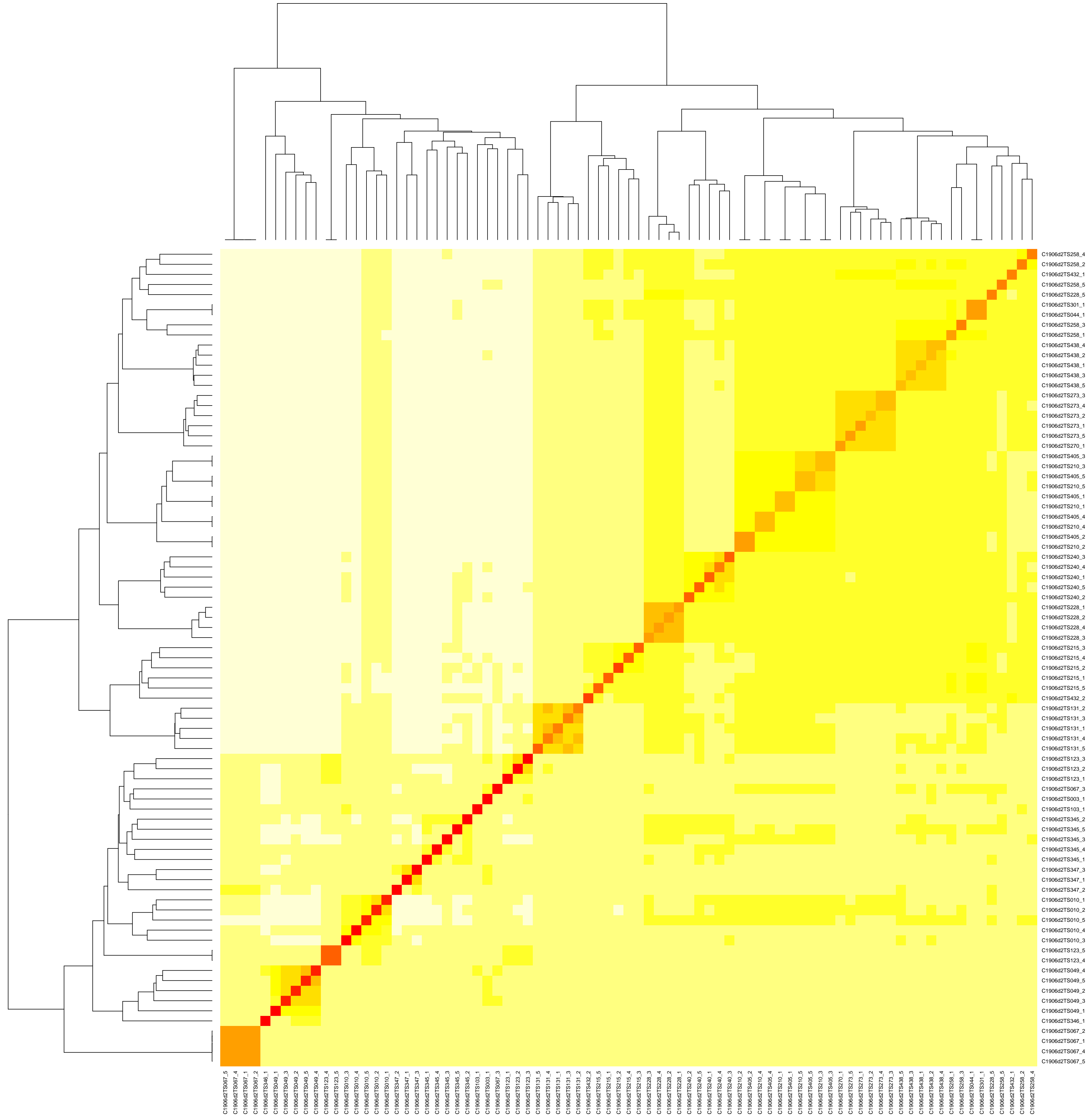
CAD-score-based clustering heatmap for C1906d2
