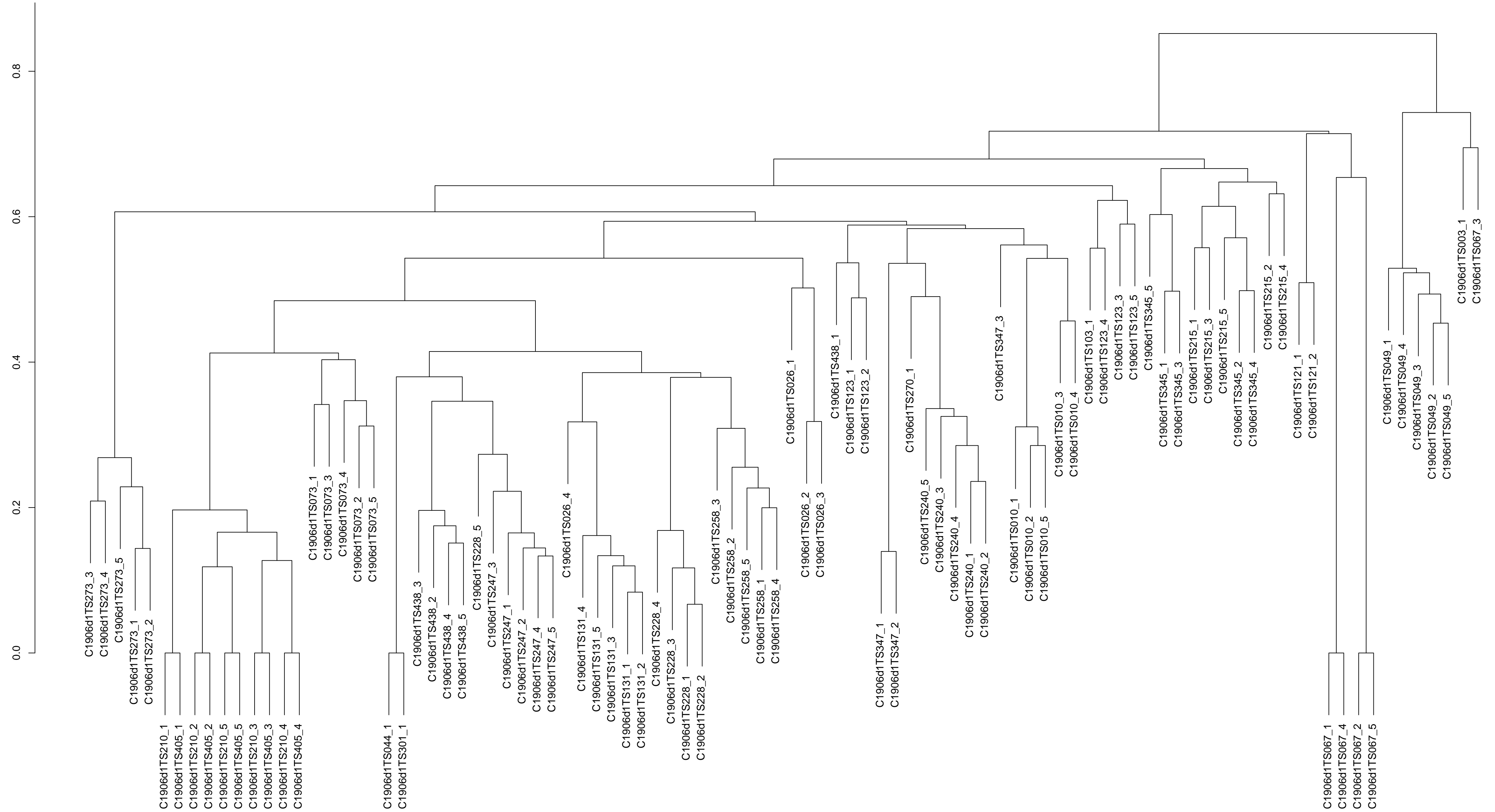
CAD-score-based clustering dendrogram for C1906d1
