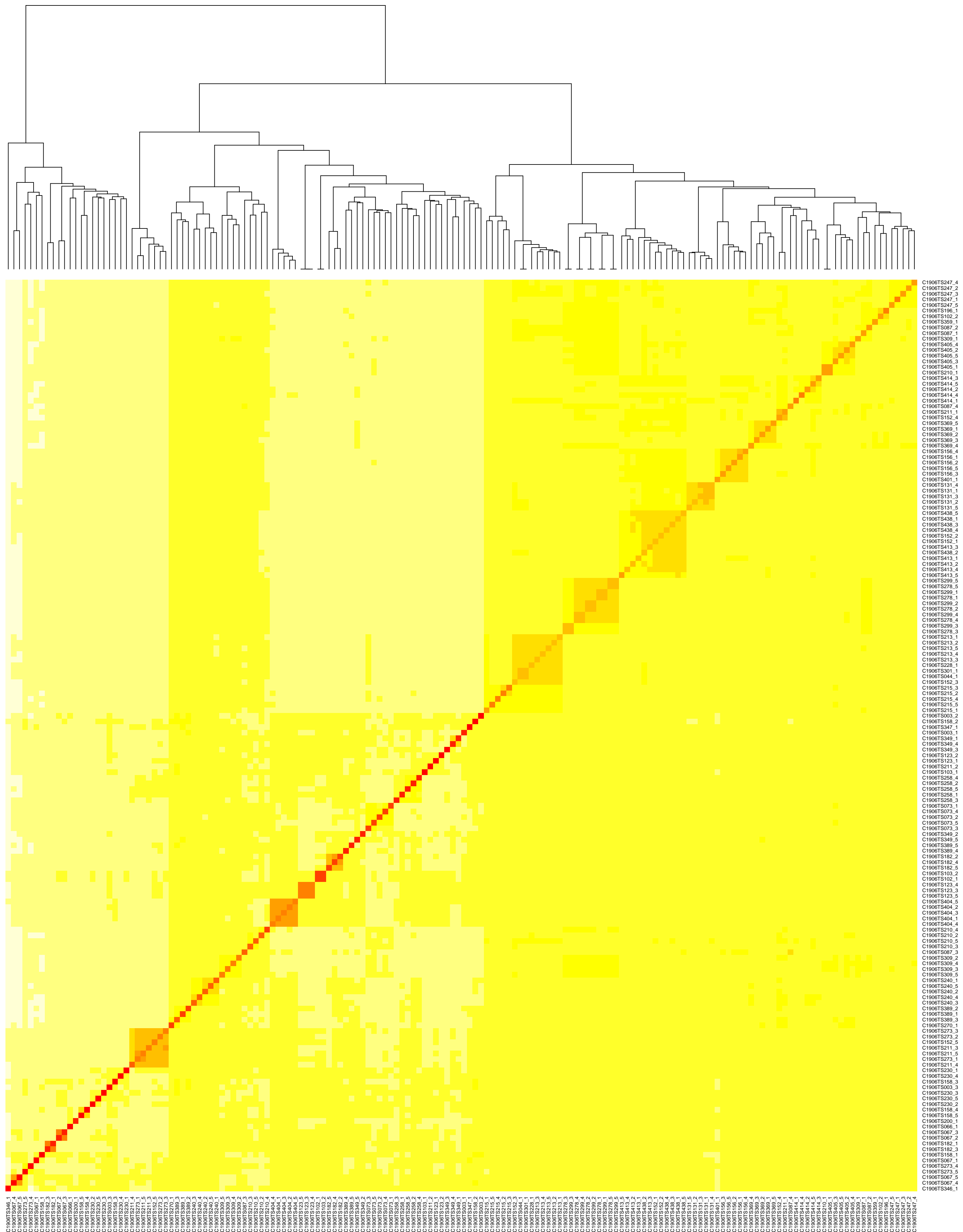
CAD-score-based clustering heatmap for C1906
