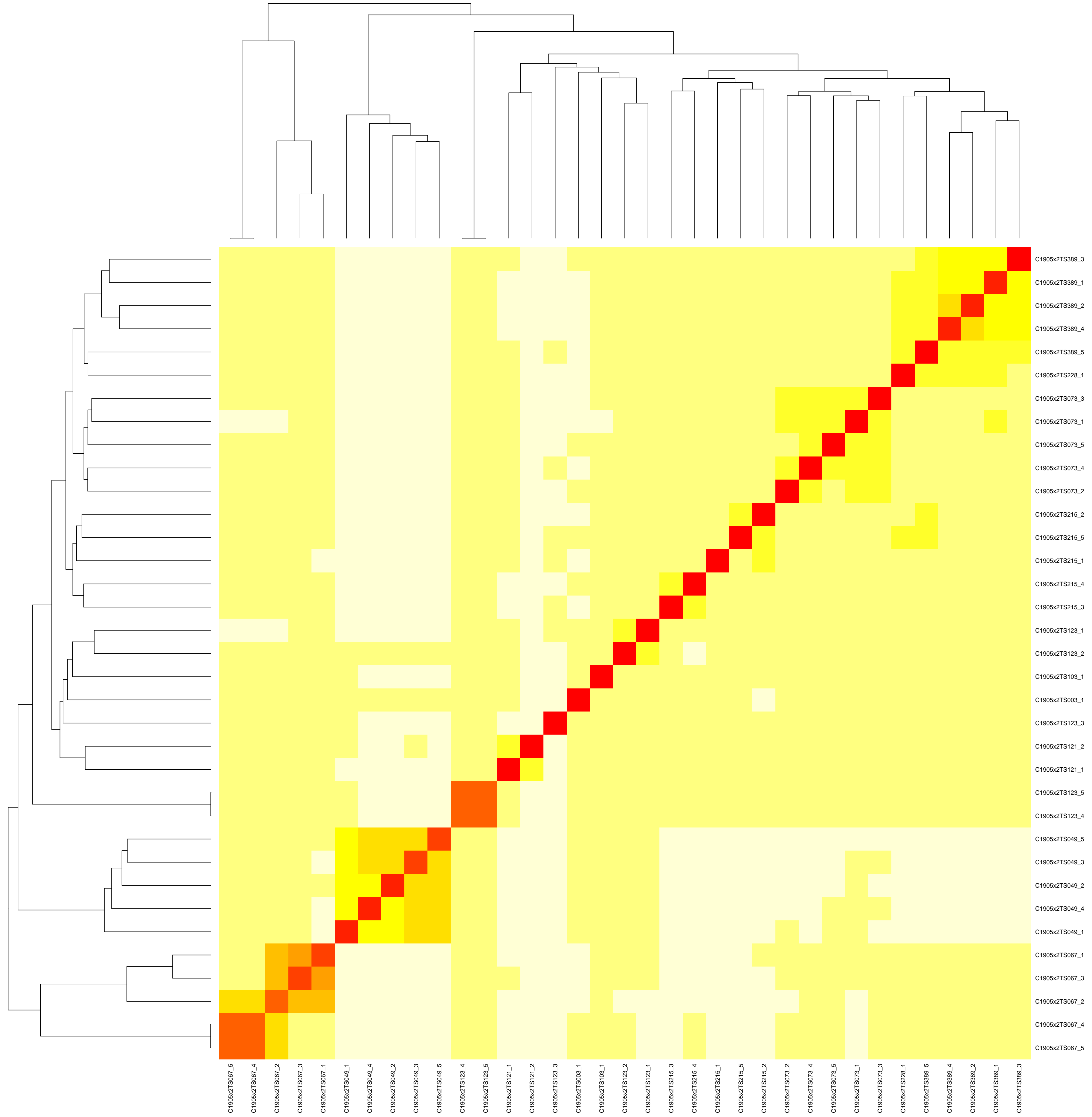
CAD-score-based clustering heatmap for C1905x2
