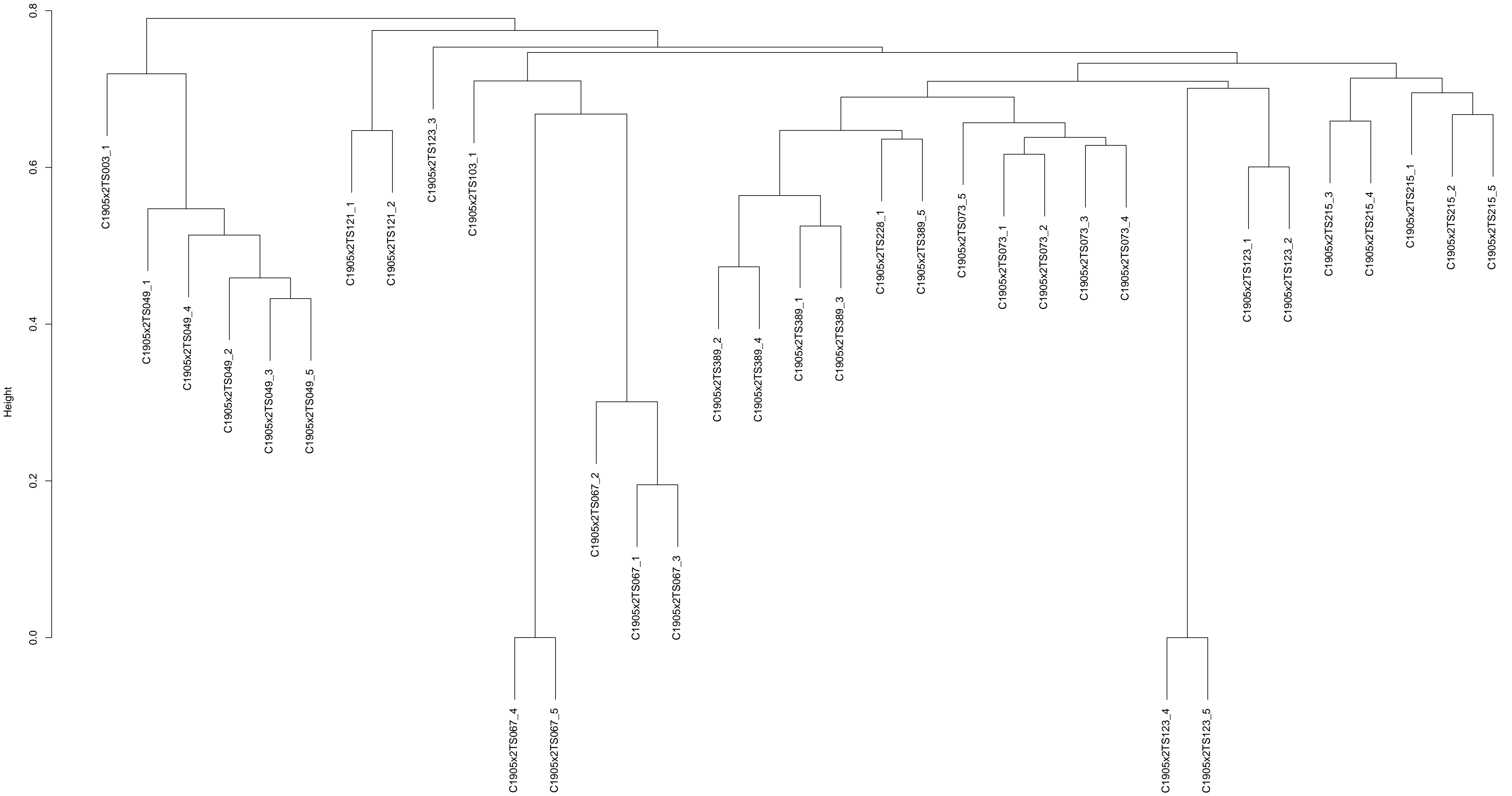
CAD-score-based clustering dendrogram for C1905x2
