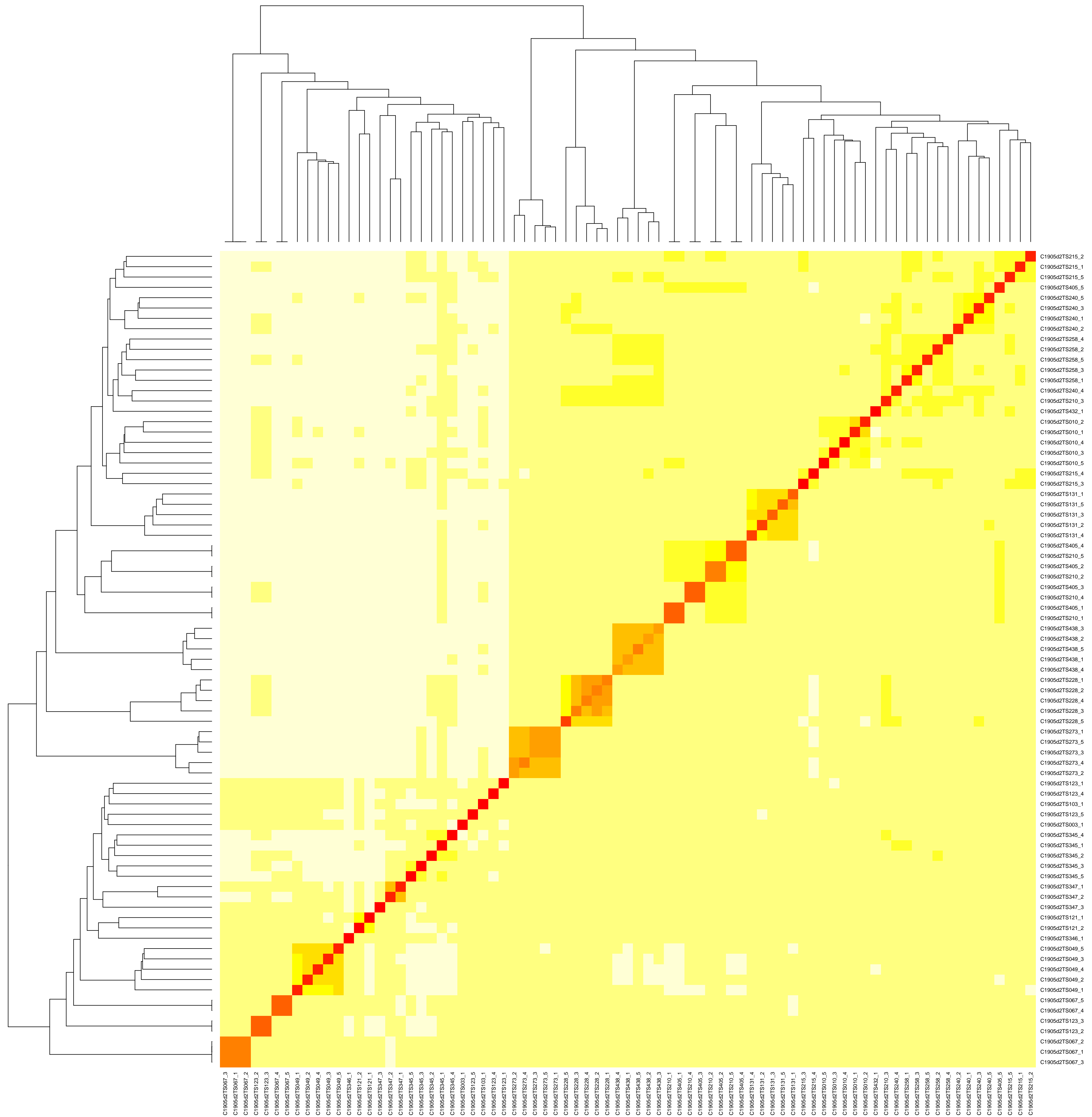
CAD-score-based clustering heatmap for C1905d2
