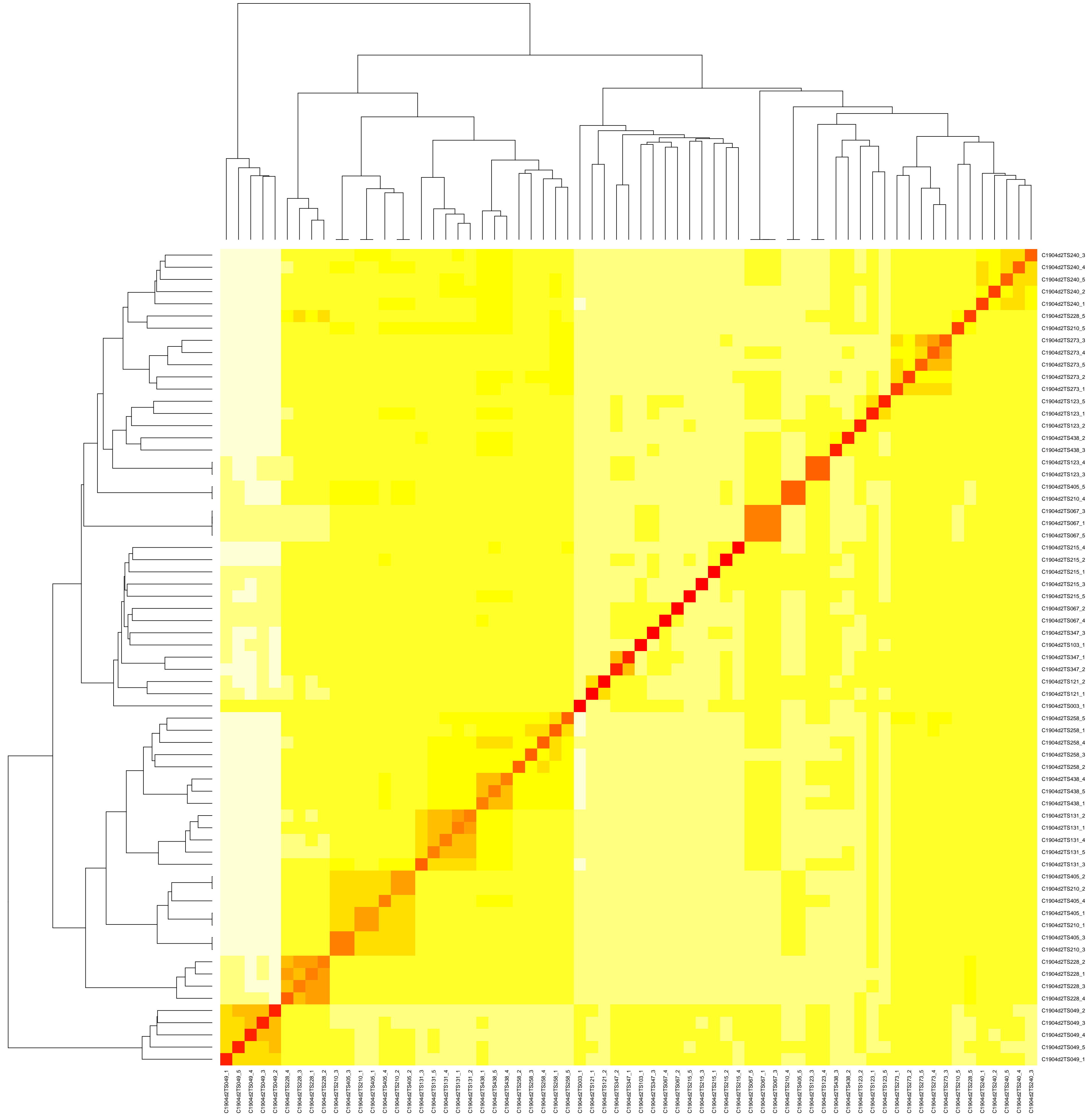
CAD-score-based clustering heatmap for C1904d2
