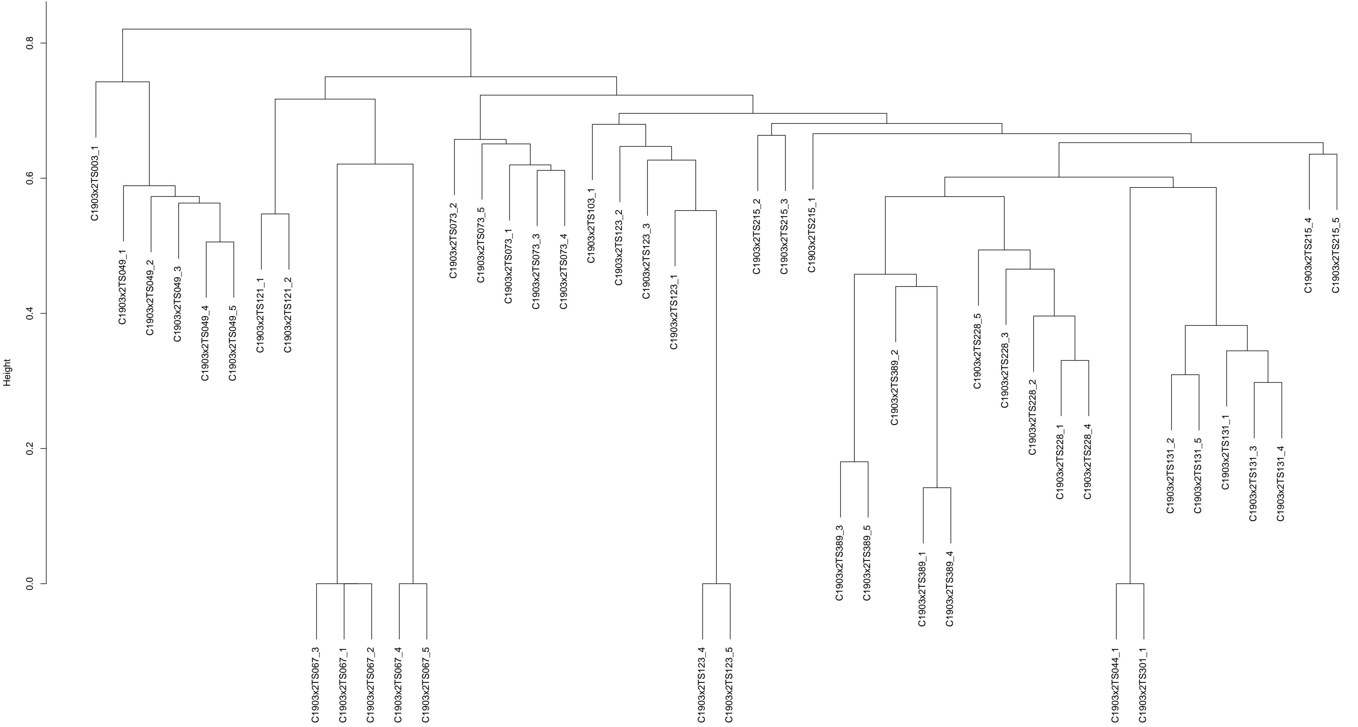
CAD-score-based clustering dendrogram for C1903x2
