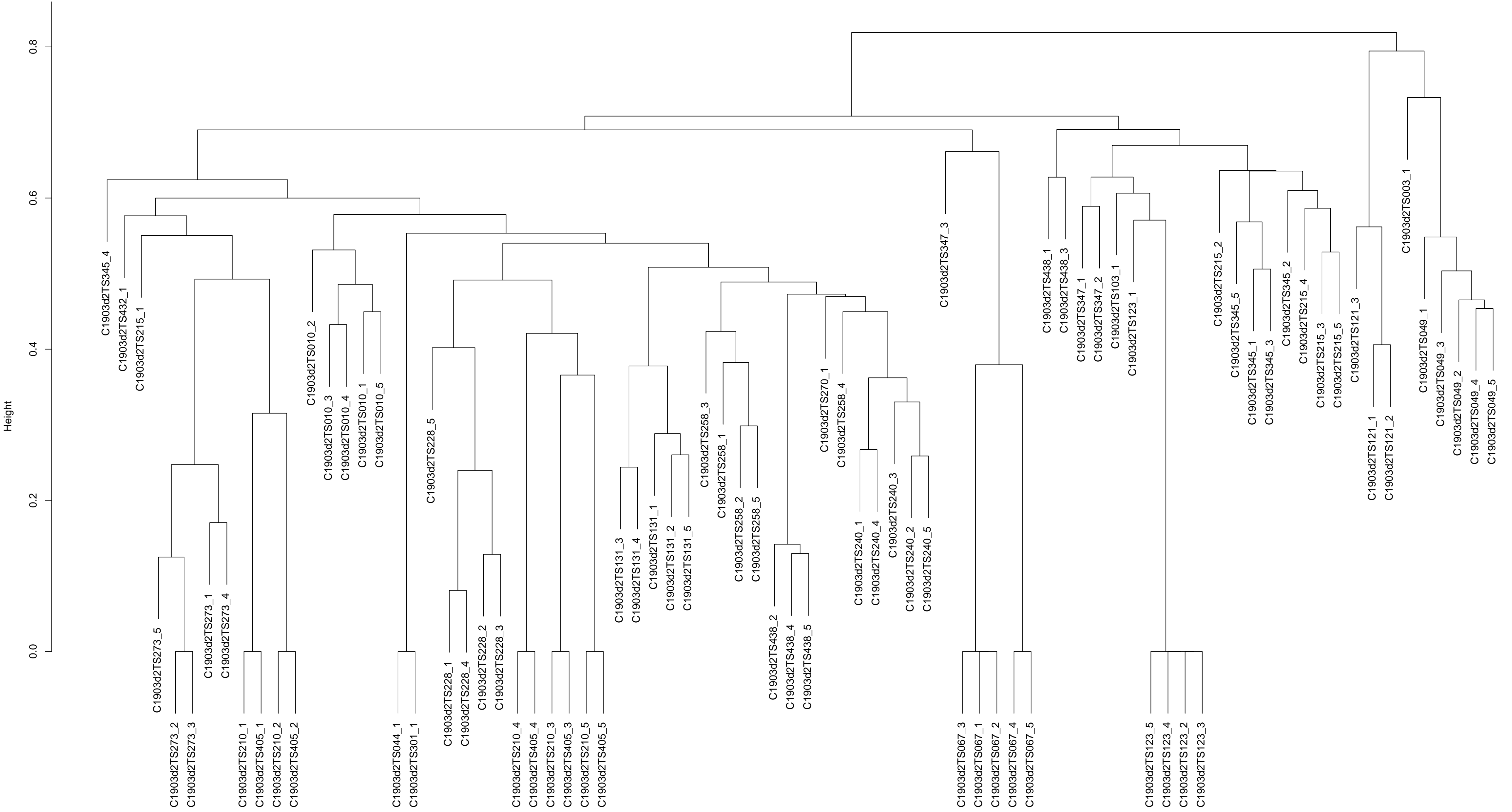
CAD-score-based clustering dendrogram for C1903d2
