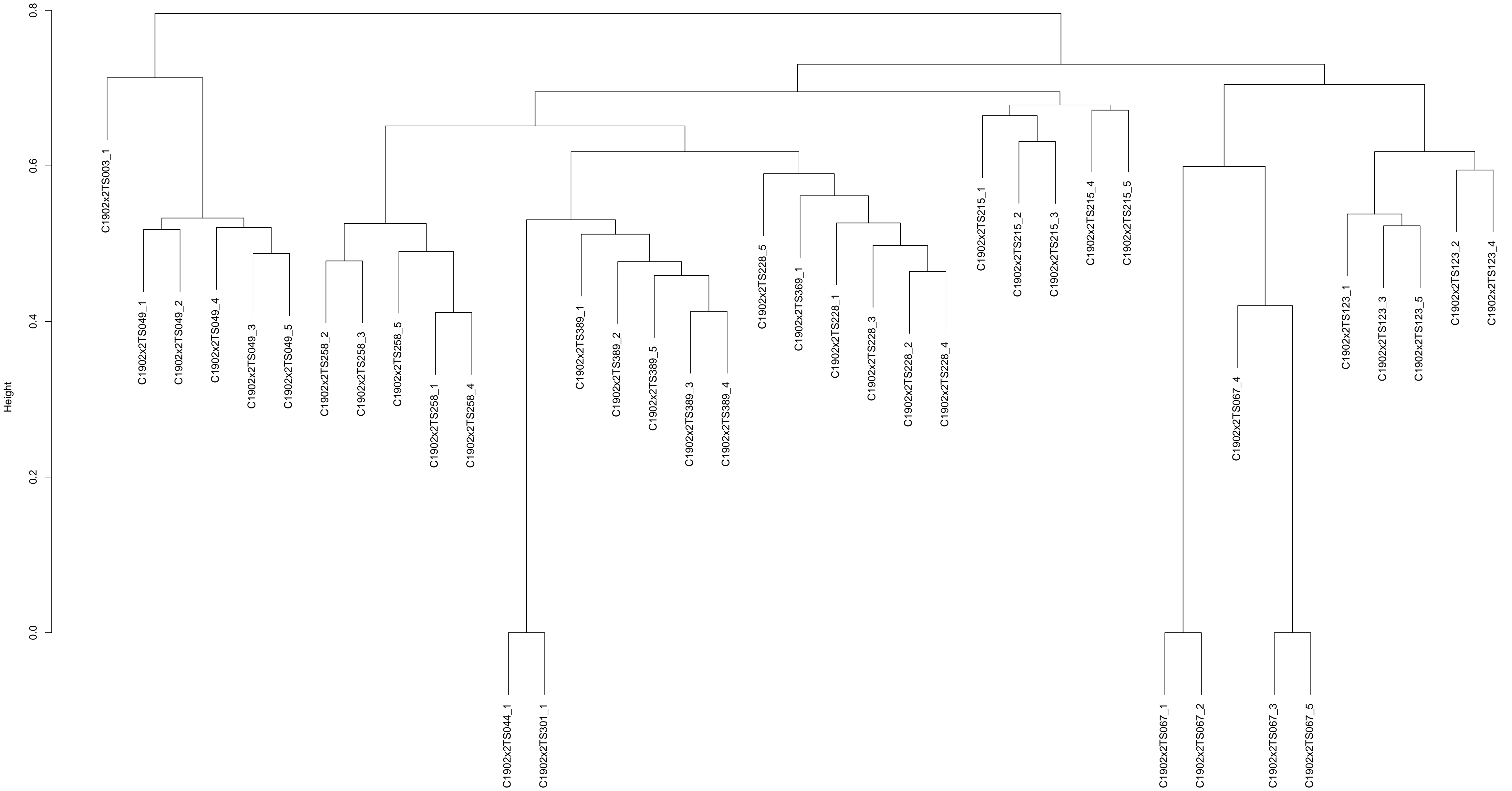
CAD-score-based clustering dendrogram for C1902x2
