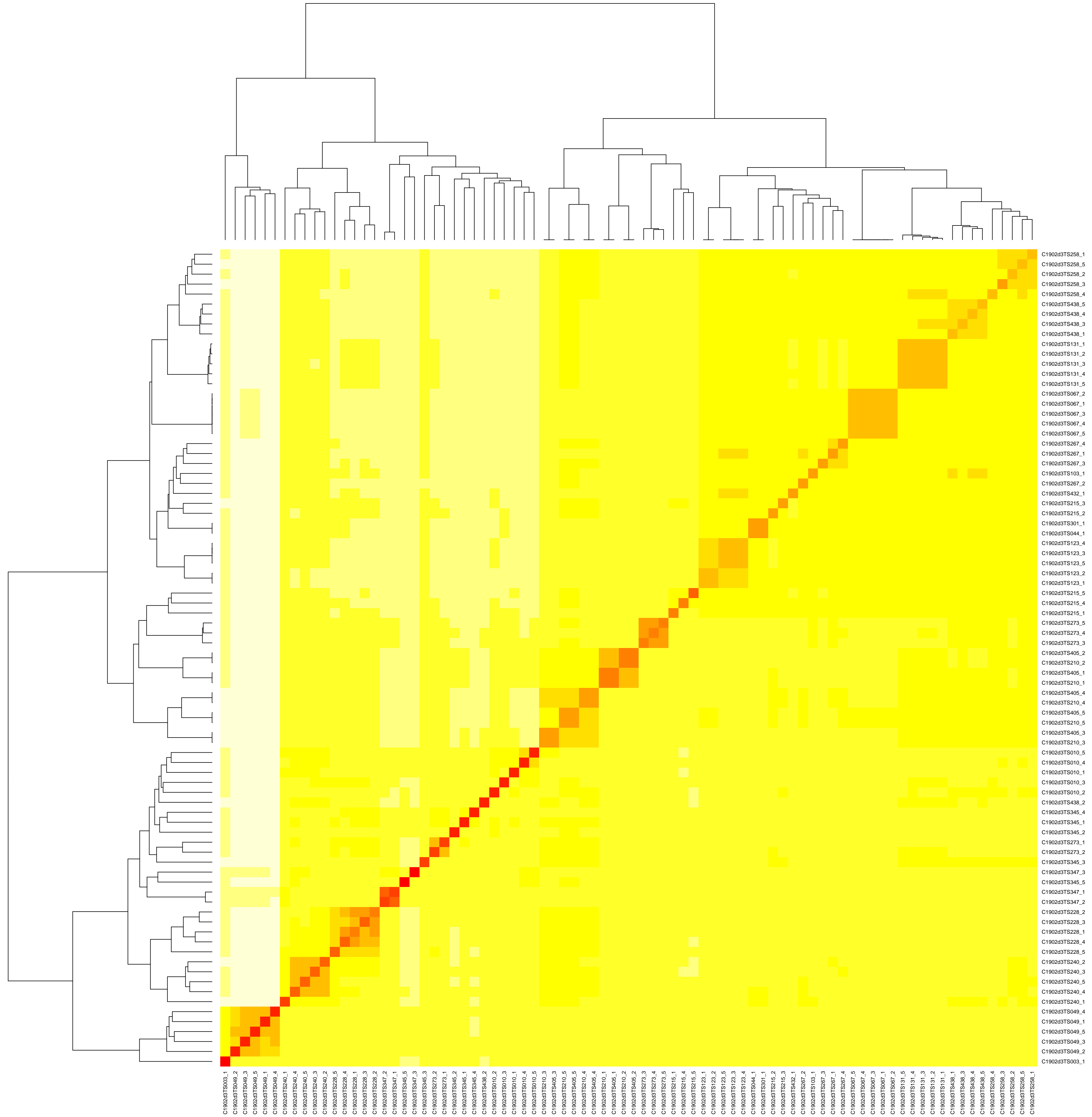
CAD-score-based clustering heatmap for C1902d3
