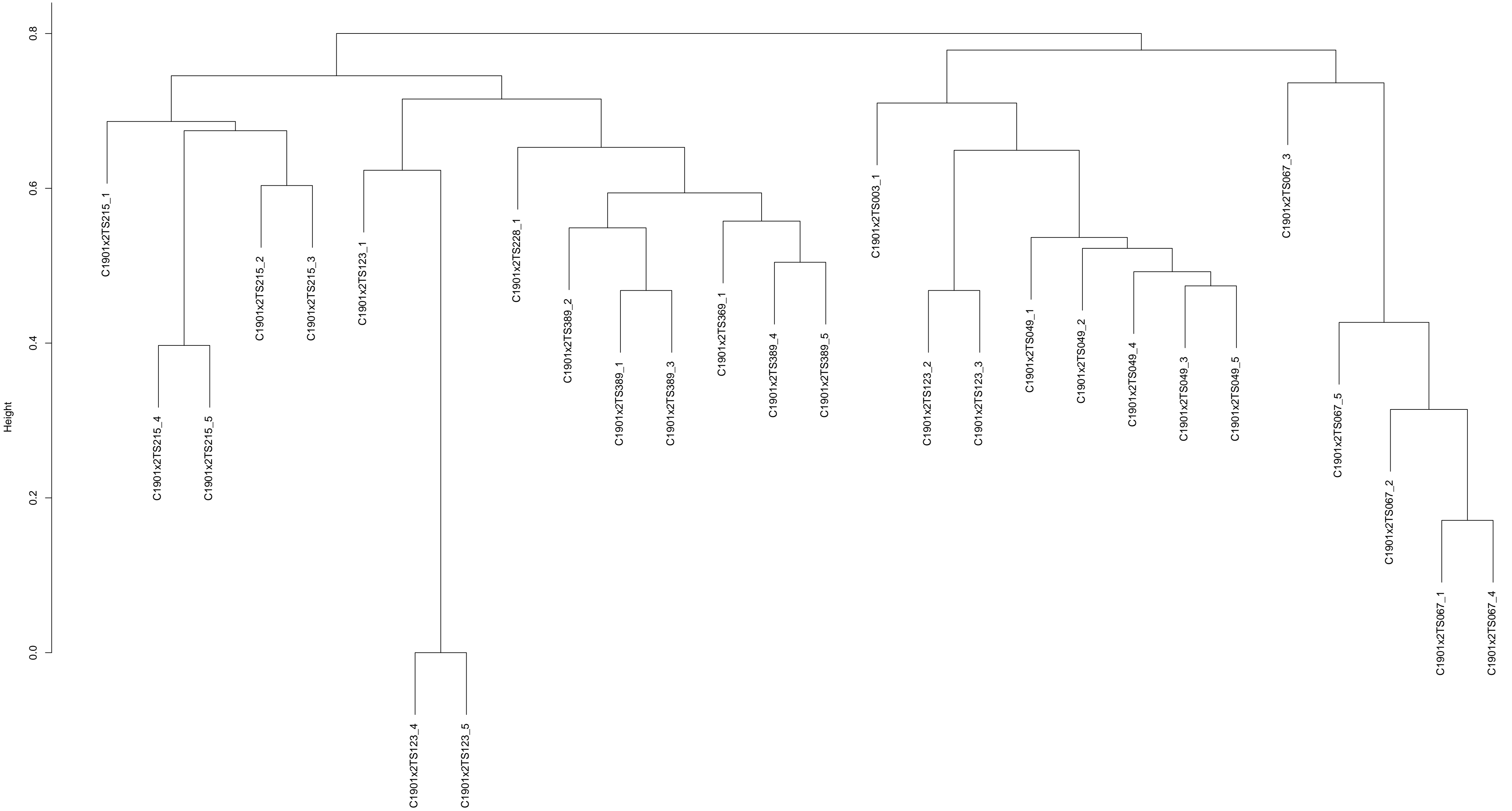
CAD-score-based clustering dendrogram for C1901x2
