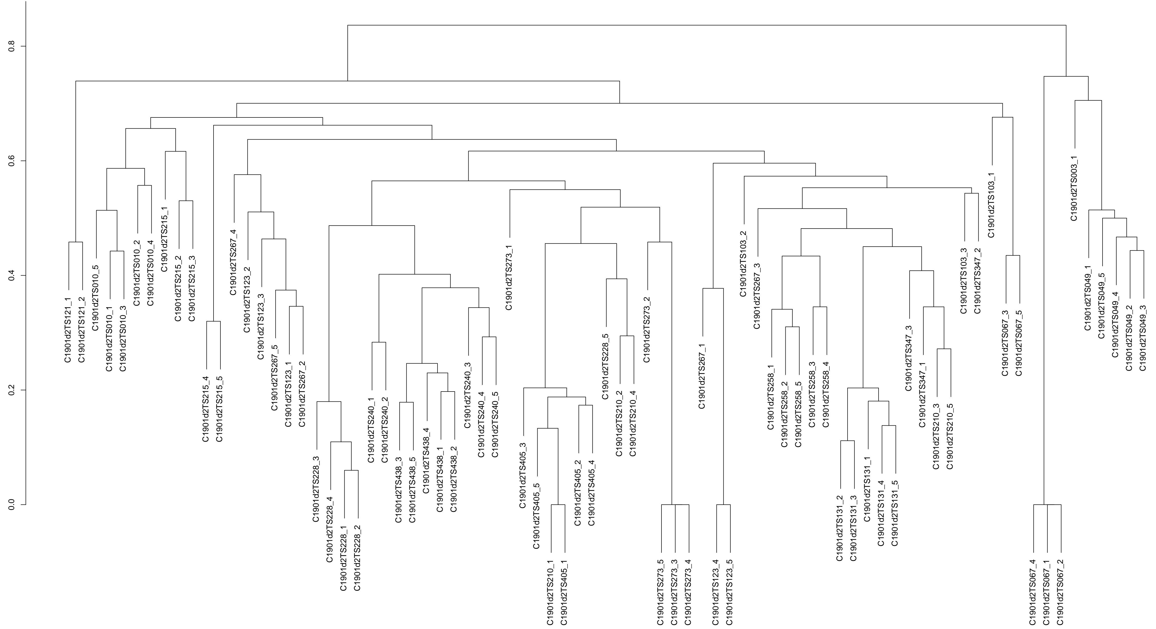
CAD-score-based clustering dendrogram for C1901d2
