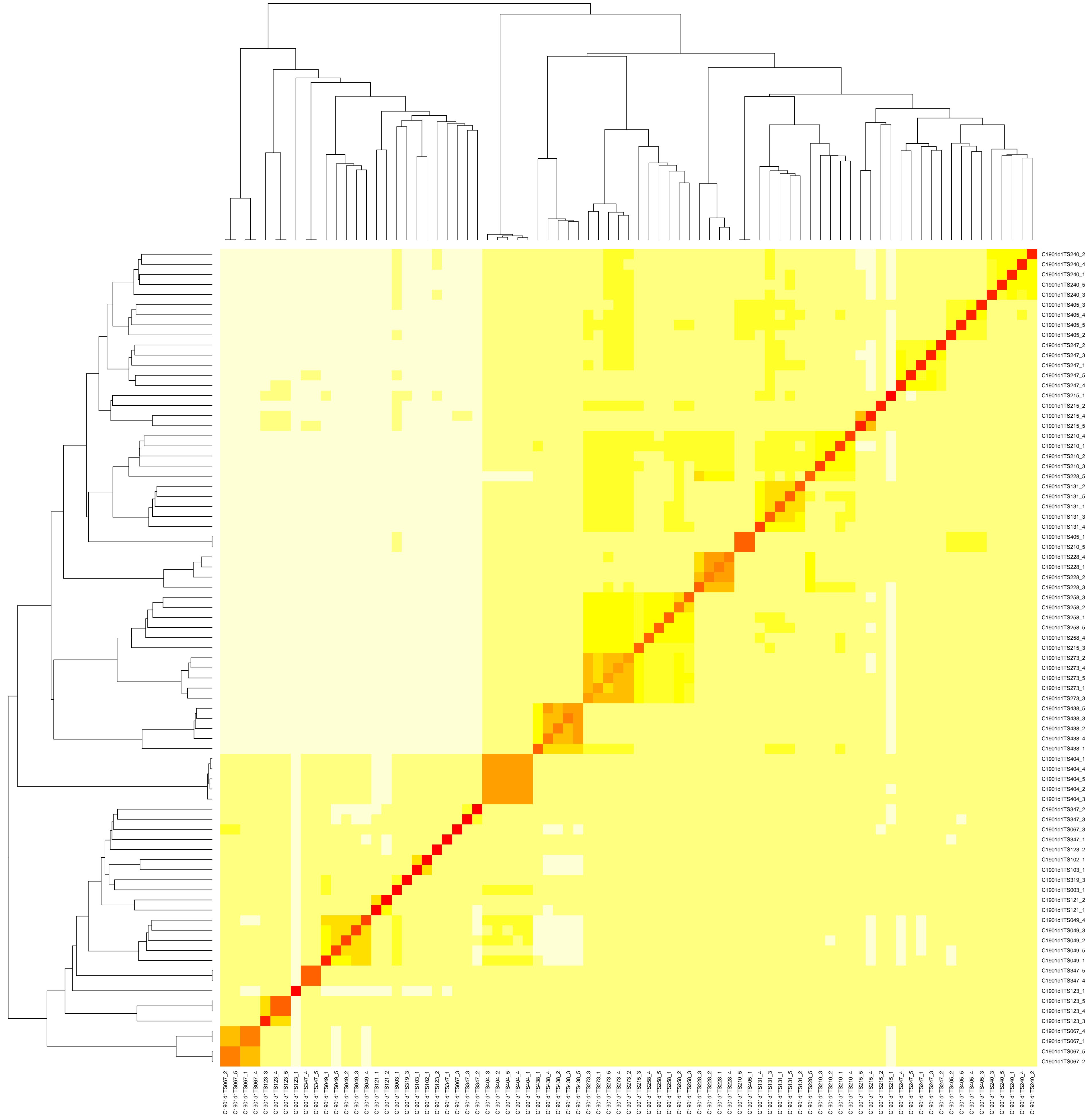
CAD-score-based clustering heatmap for C1901d1
